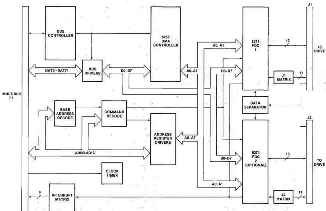
Figure 1. iSBC 204 Single Density Diskette Controller Block Diagram
