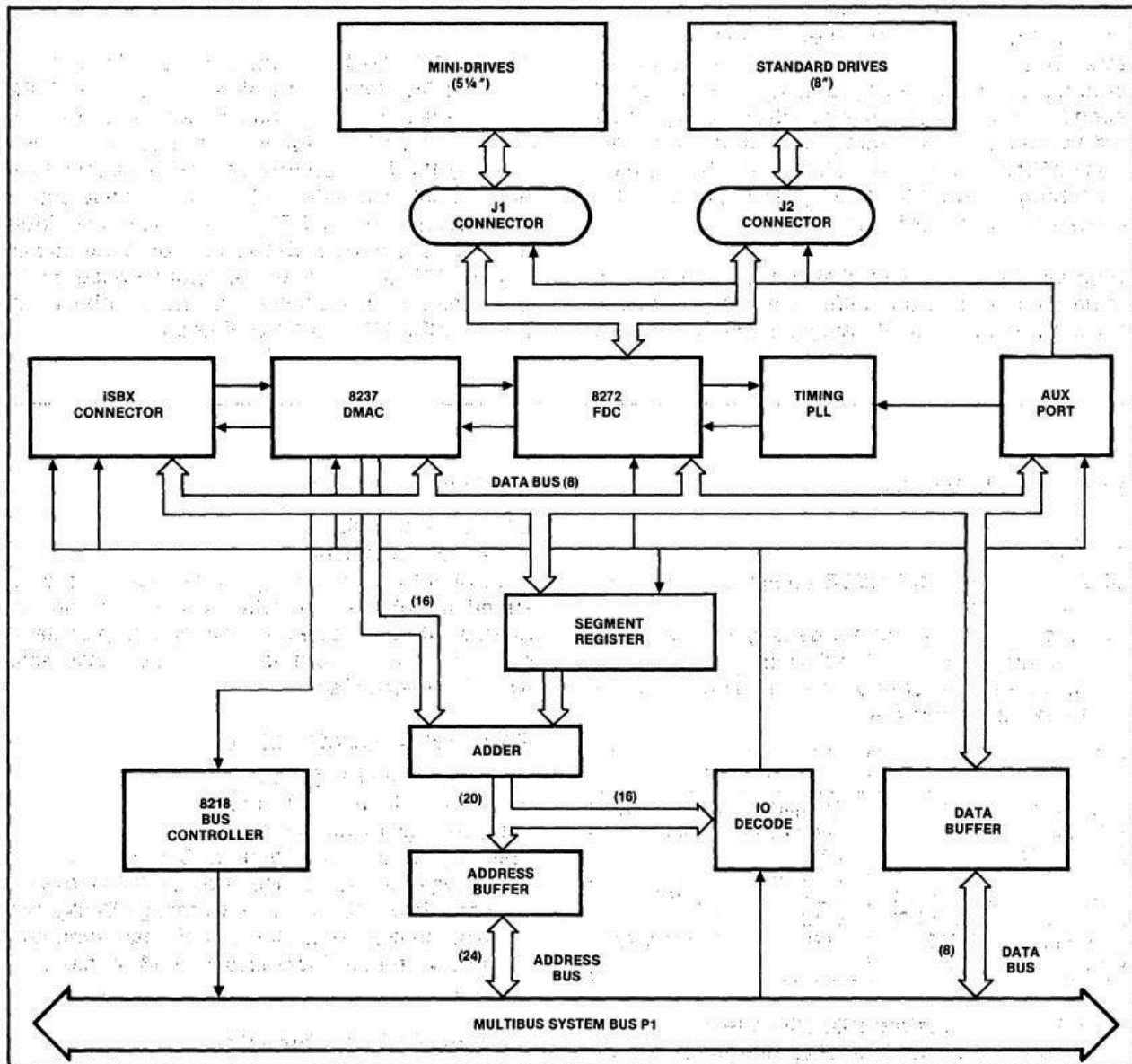
Figure 1. ISBC 208 Flexible Disk Controller Block Diagram
