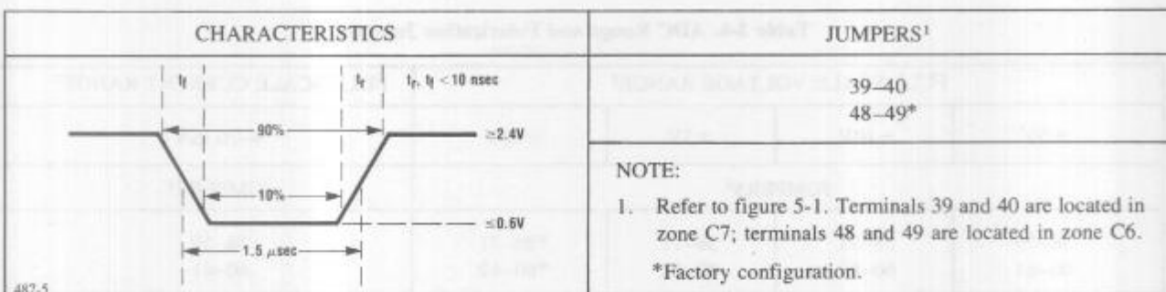
Figure 2-4. External TADC/ Clock Characteristics and Jumpers
