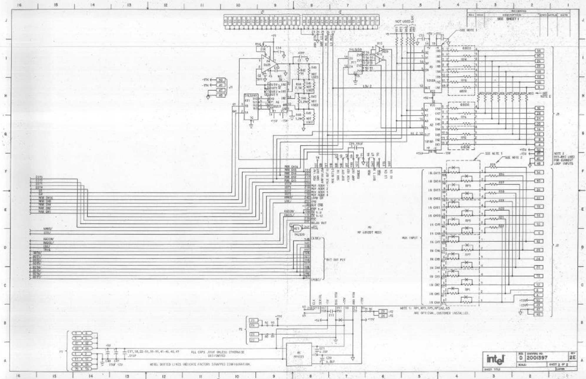
Figure 5-2. SBC 711 Schematic Diagram (Sheet 2 of 2)
