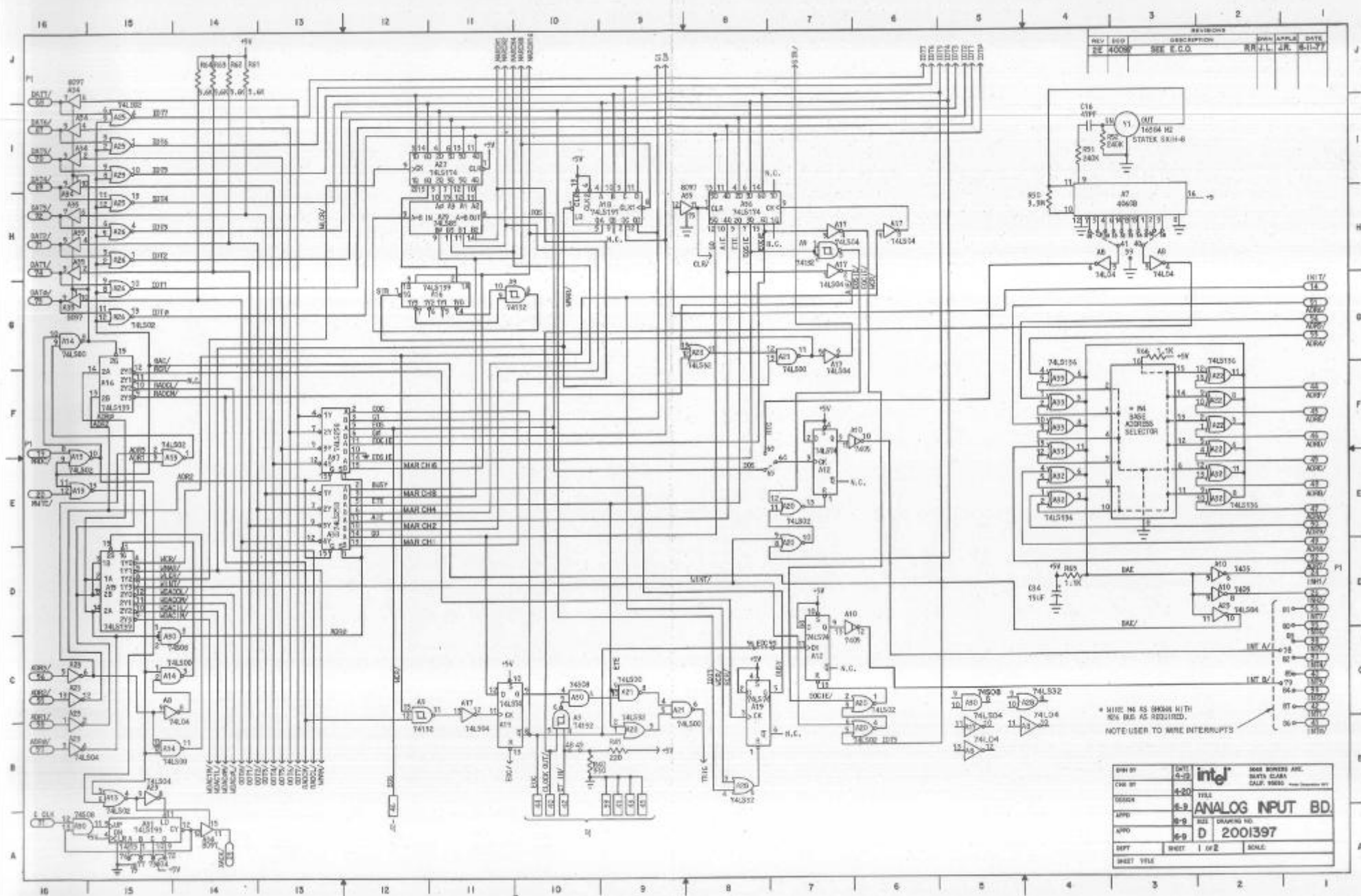
Figure 5-2. SBC 711 Schematic Diagram (Sheet 1 of 2)
